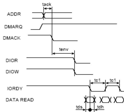
Figure 14. UDMA In Transfer Starts Timing Diagram
