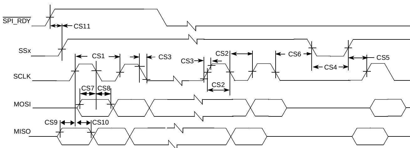
Figure 20. CSPI Master Mode Timing Diagram
