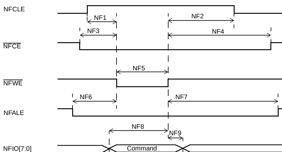
Figure 22. Command Latch Cycle Timing Diagram
