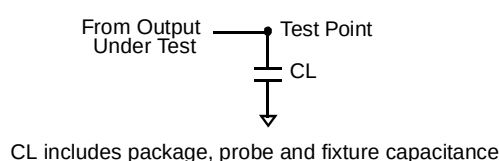
Figure 4. Load Circuit for Output
