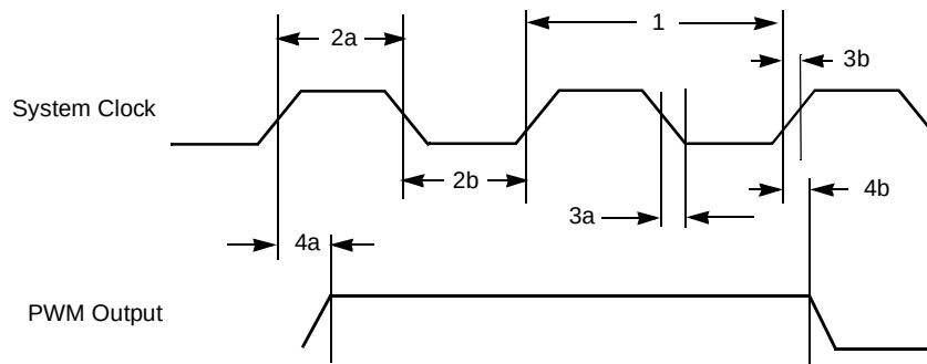
Figure 70. PWM Timing
