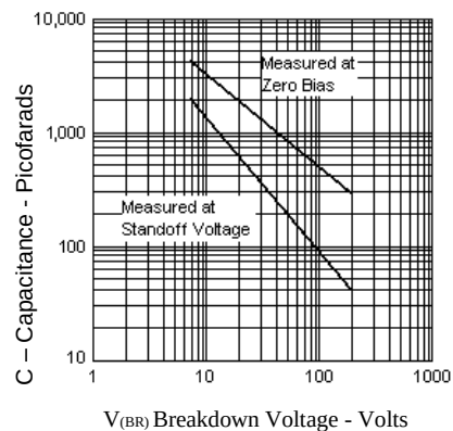
FIGURE 4 – P6KE Typical Capacitance vs. Breakdown Voltage
