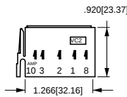
MARKING DETAIL FRONT VIEW VC2 CONNECTOR HOUSING (For AMP terminals only)
