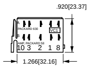
MARKING DETAIL FRONT VIEW VC1 CONNECTOR HOUSING
