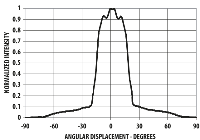
Figure 7. Representative spatial radiation pattern for 30° viewing angle lamps
