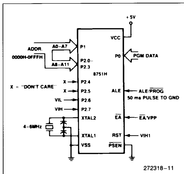
Figure 5. Programming Configuration
