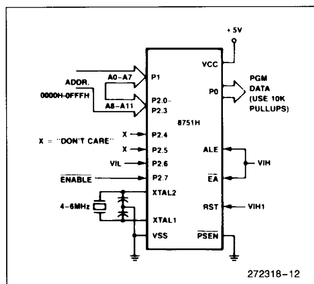
Figure 6. Program Verification
