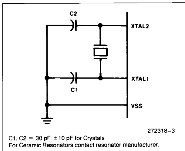
Figure 3. Oscillator Connections
