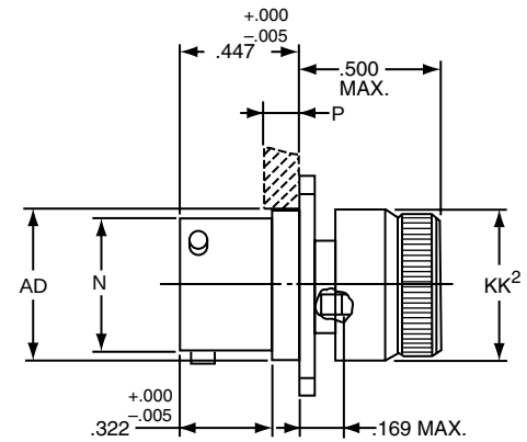
* JTPQ00RE-XX-XXX (MS27497E)
