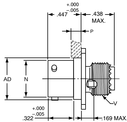
* JTPQ00RT-XX-XXX (MS27497T) ** JTPSQ00RT-XX-XXX
