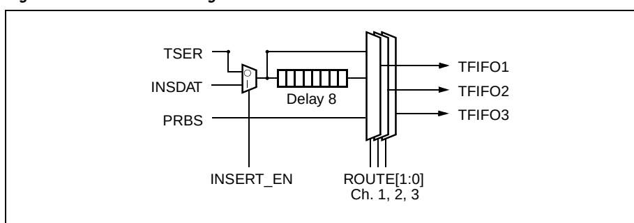
Figure 4-1. Transmit Routing
