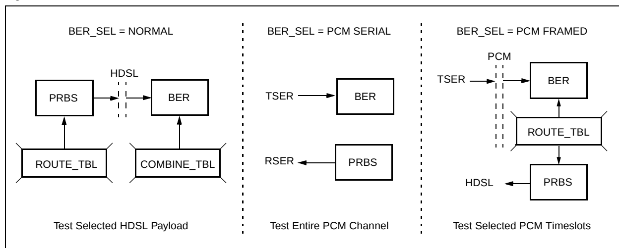
Figure 3-12. PRBS/BER Measurements
