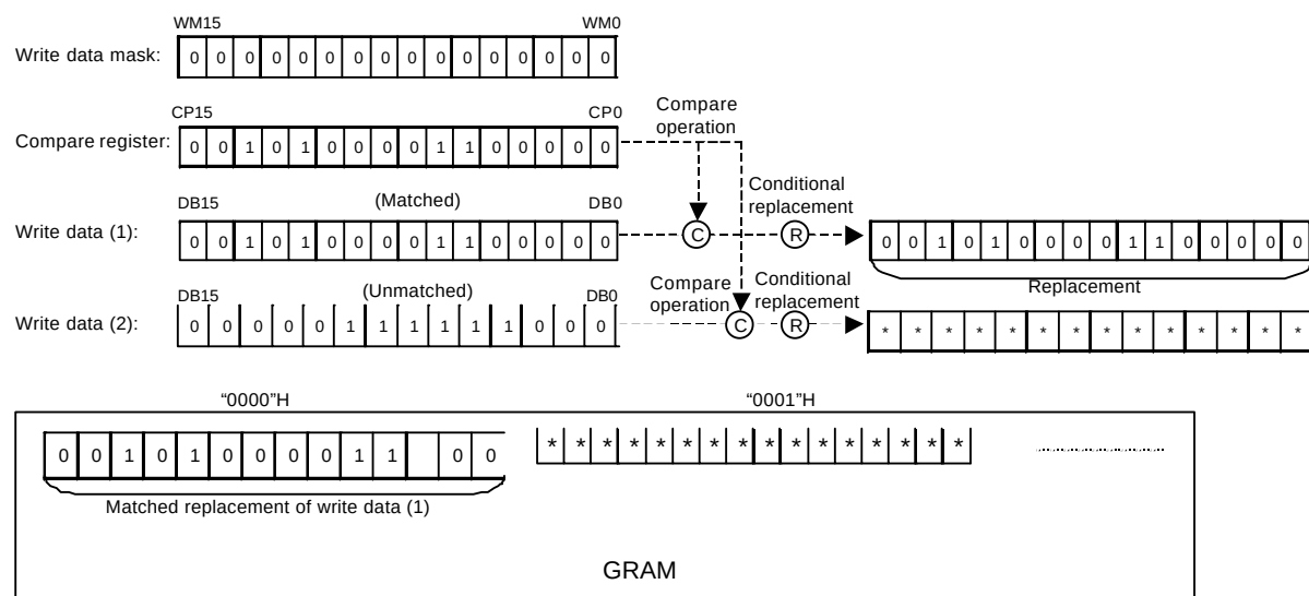
Figure 29. Writing operation write mode 3
