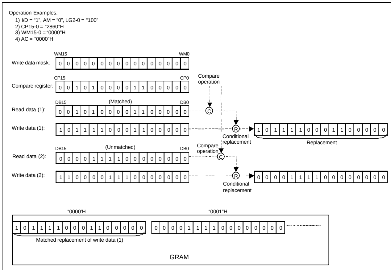
Figure 33. Writing operation of read/write mode 3
