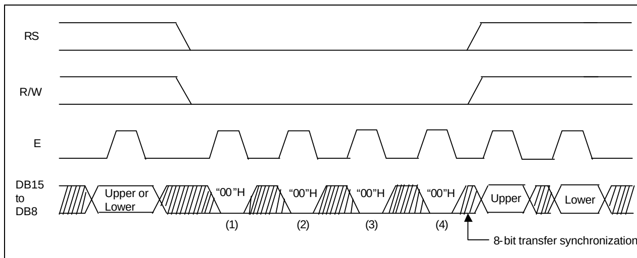
Figure 19. 8-bit transfer synchronization
