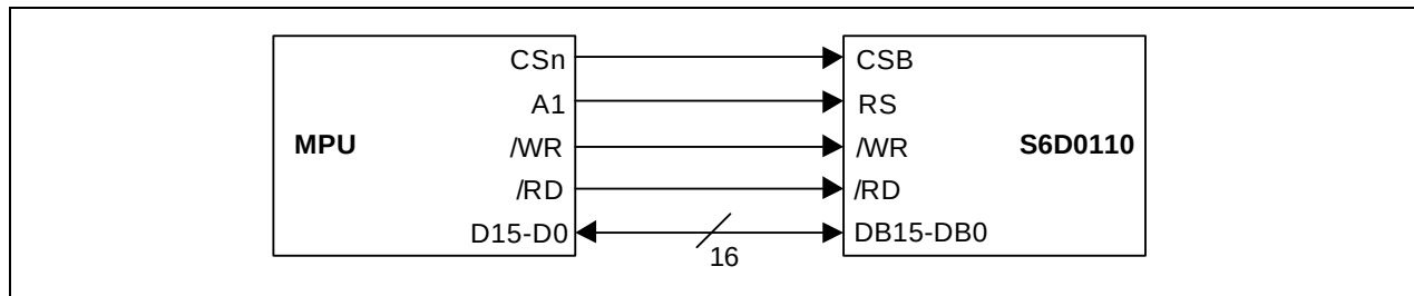
Figure 17. Interface to 16-bit microcomputer
