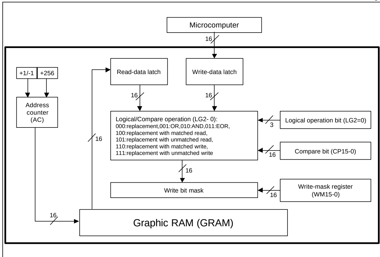
Figure 25. Data processing flow of graphic operation
