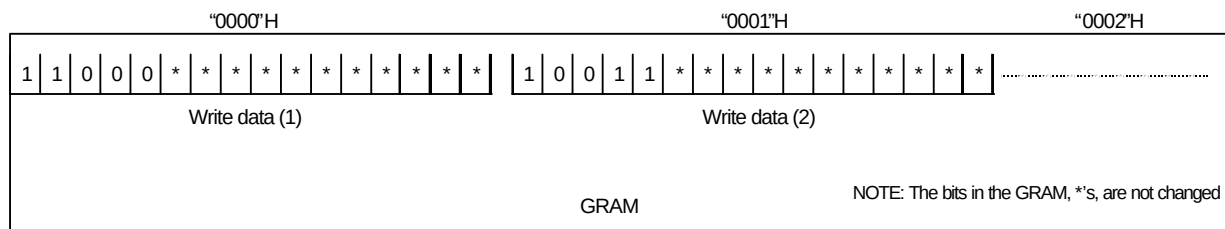
Figure 27. Writing operation of write mode 1
