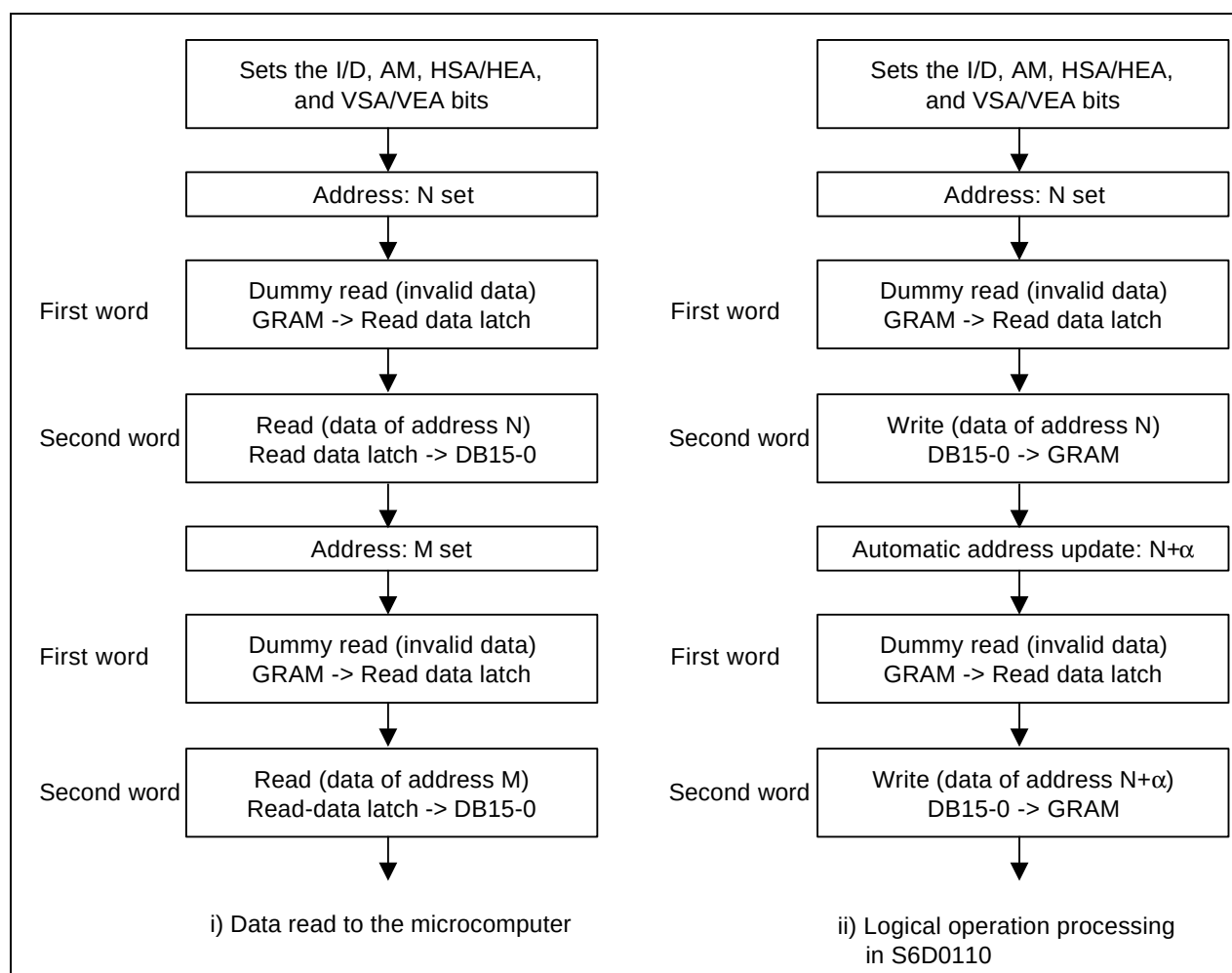
Figure 16. GRAM read sequence
