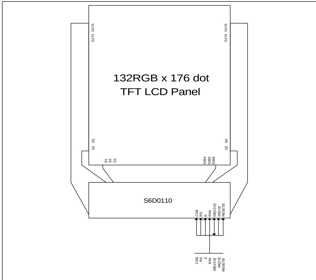
Figure 44. System structure
