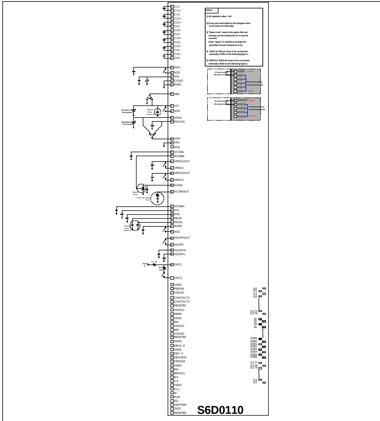
Figure 54. Application Circuit
