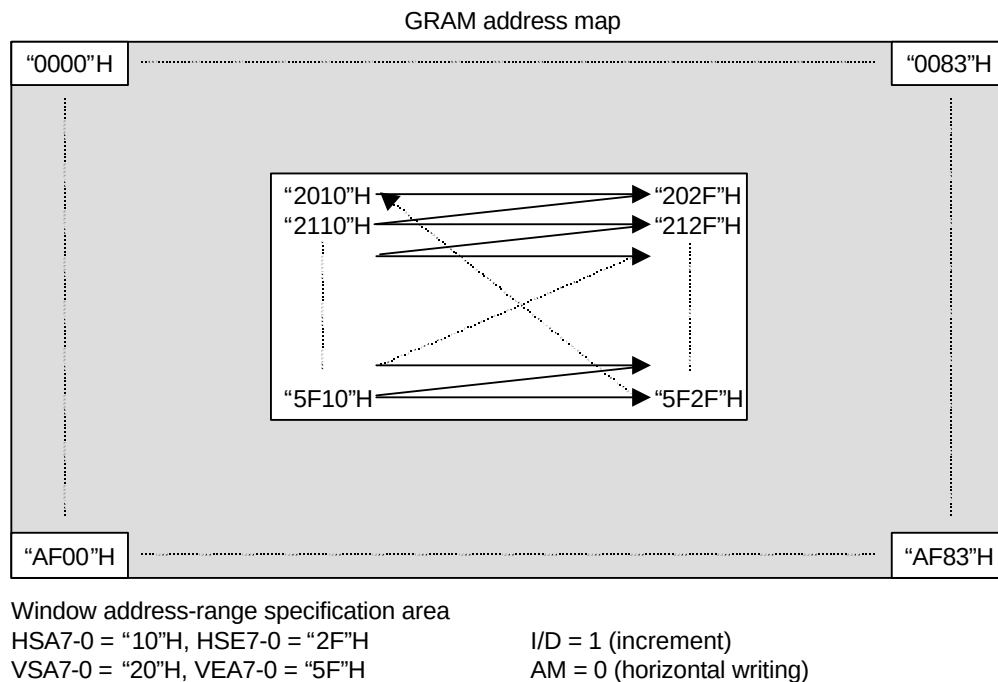
Figure 24. Example of address operation in the window address specification
