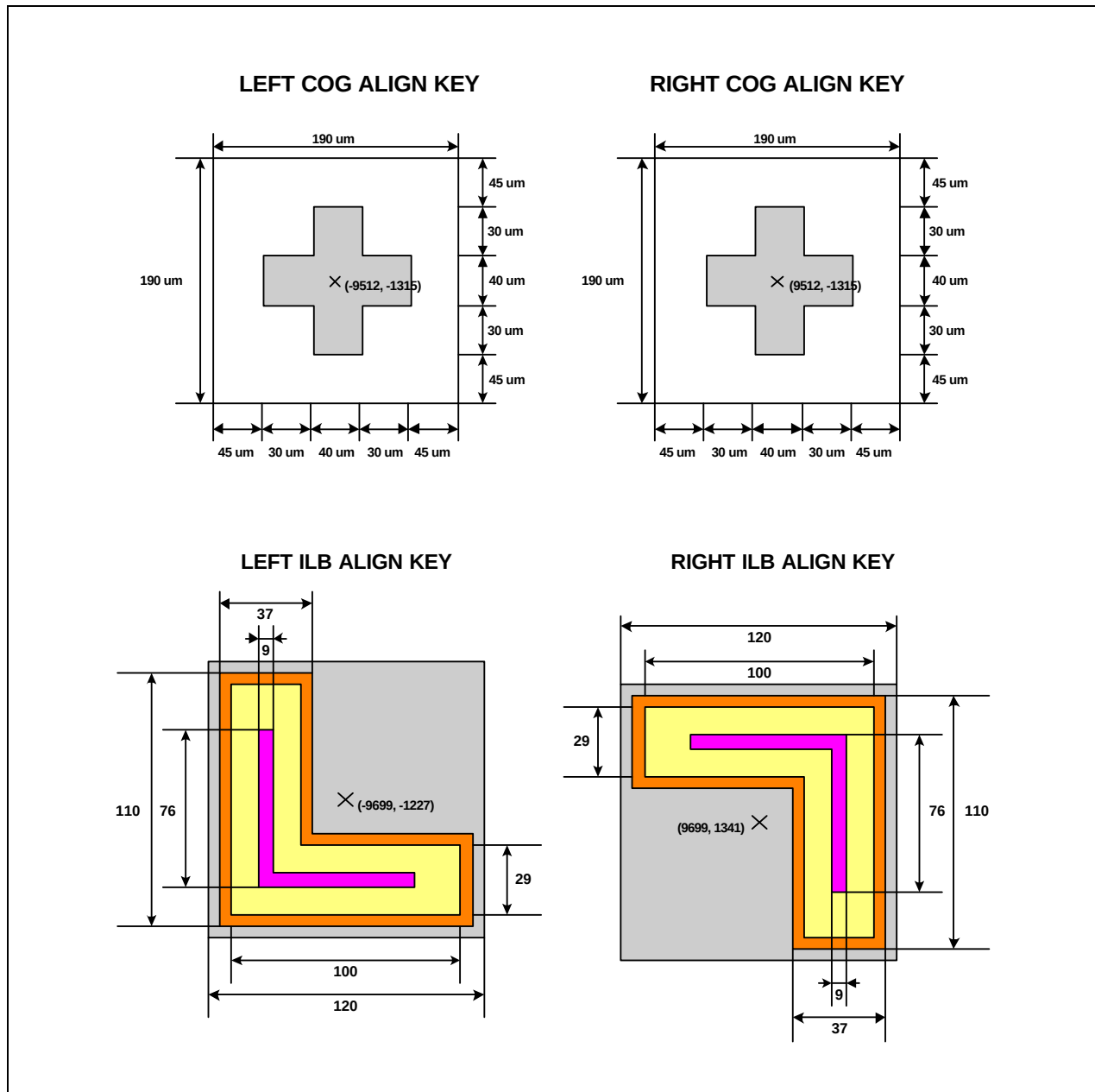
Figure 3. COG and ILB align key
