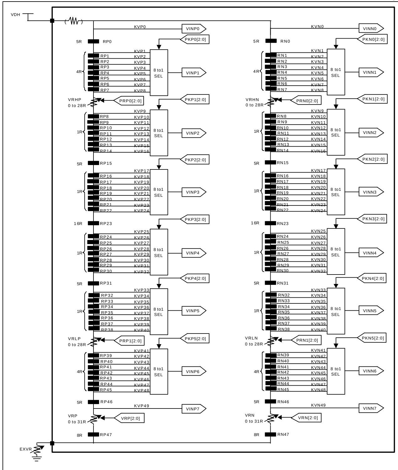
Figure 38. Structure of Ladder/8 to 1 selector
