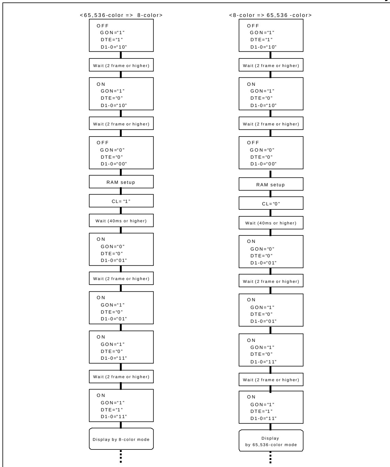
Figure 43. Set up procedure for the 8-color mode
