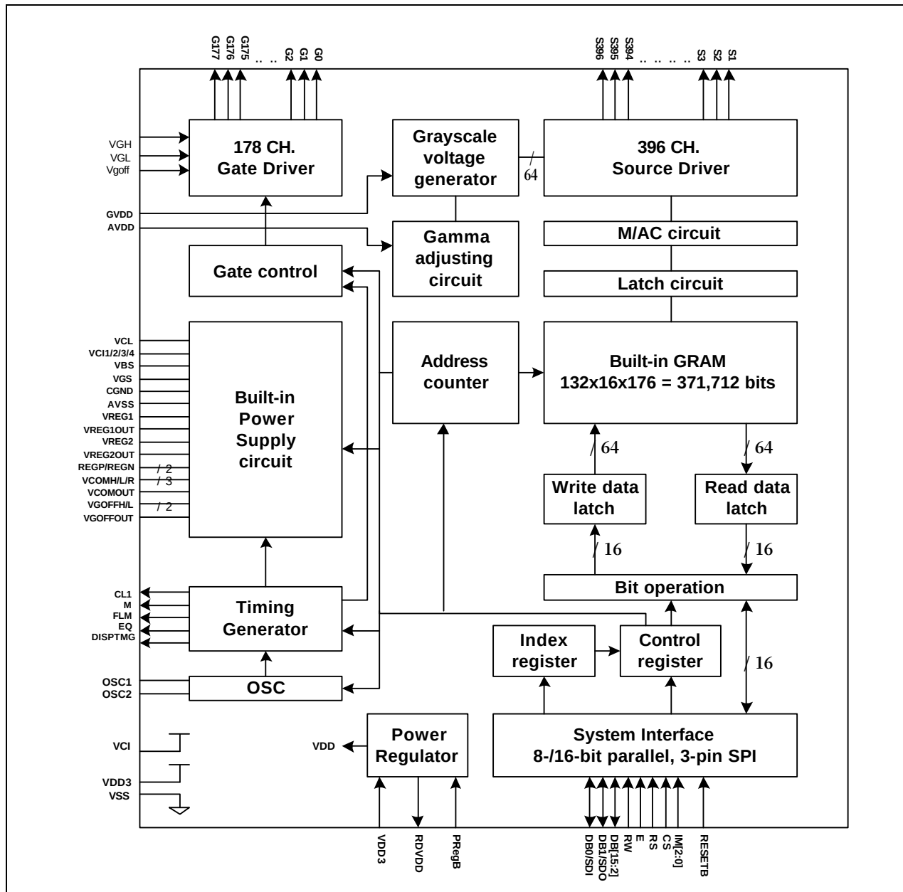
Figure 1. Block Diagram
