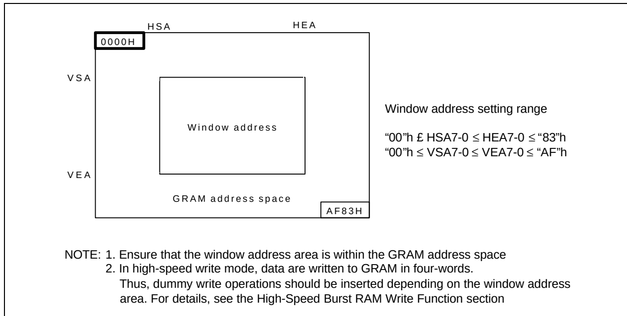
Figure 14. Window address setting range
