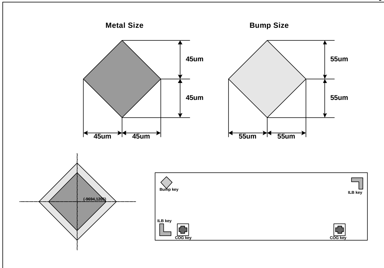
Figure 4. Bump align key and align key configuration
