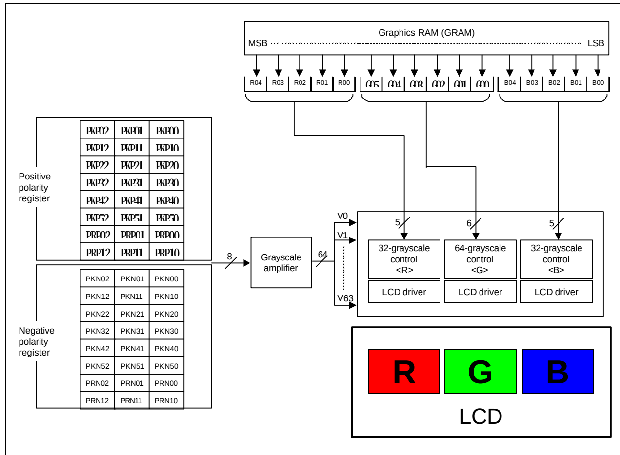
Figure 36. Grayscale control
