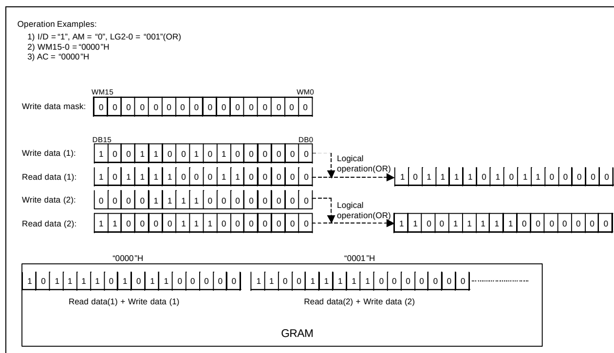
Figure 31. Writing operation of read/write mode 1
