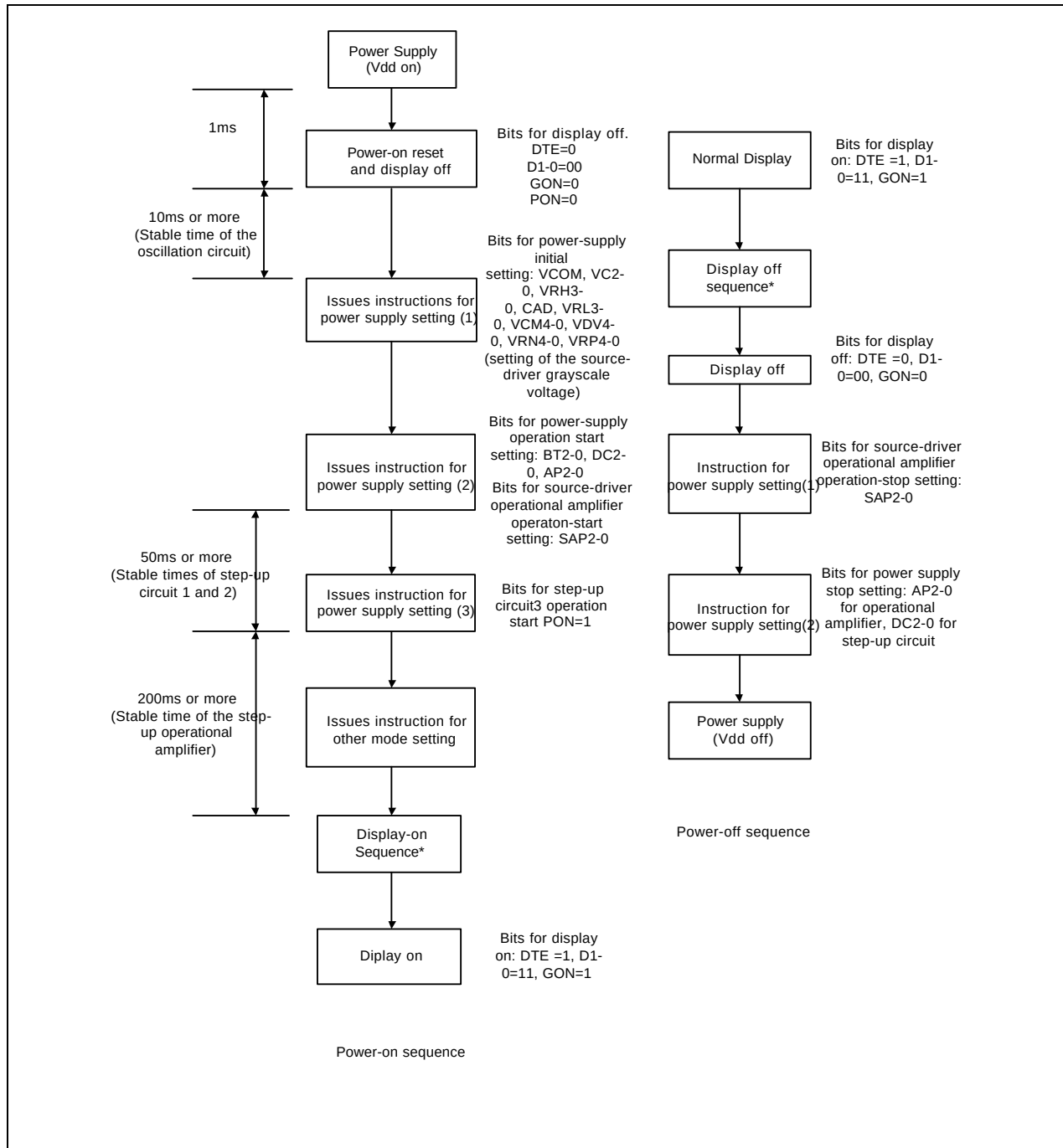
Figure 7. Set up Flow of Power Supply
