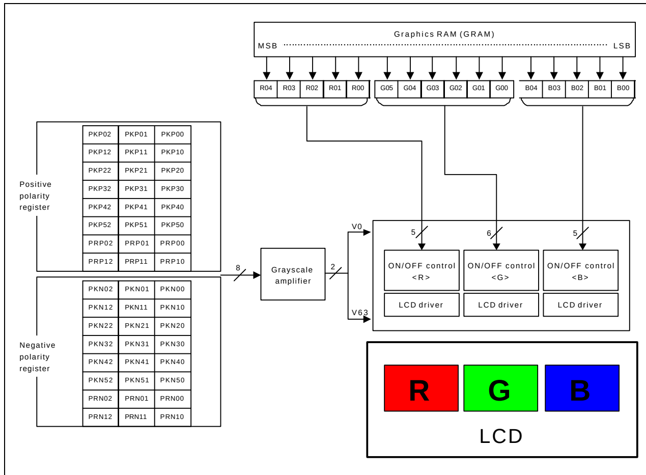
Figure 42. 8-color display control
