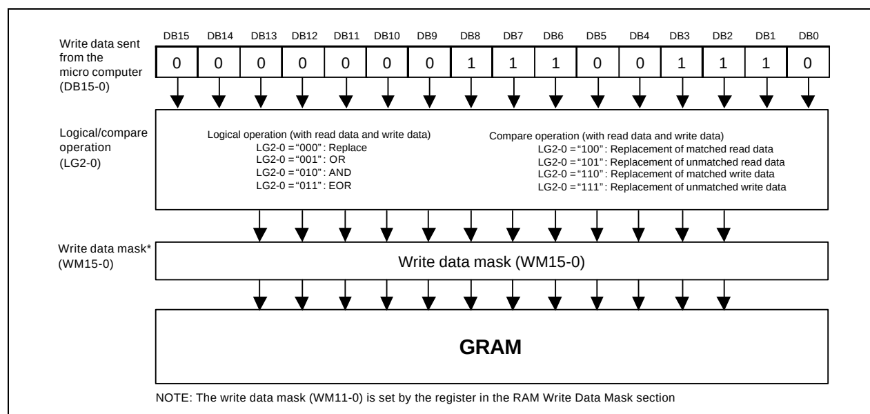
Figure 9. Logical/compare operation
