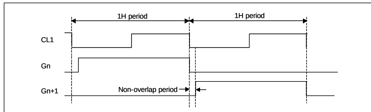
Figure 12. Non-overlap Period
