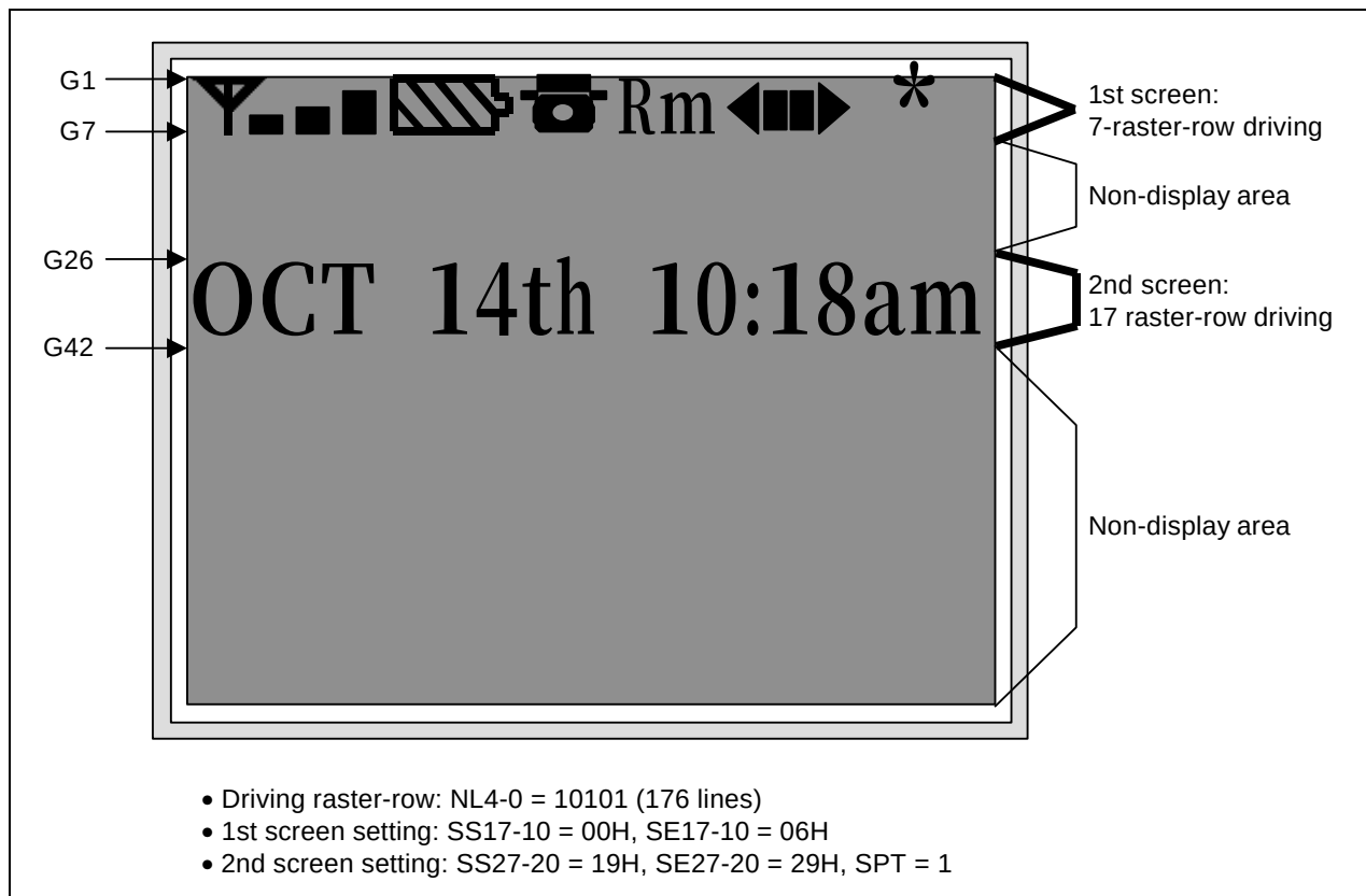
Figure 52. Driving on 2 screen
