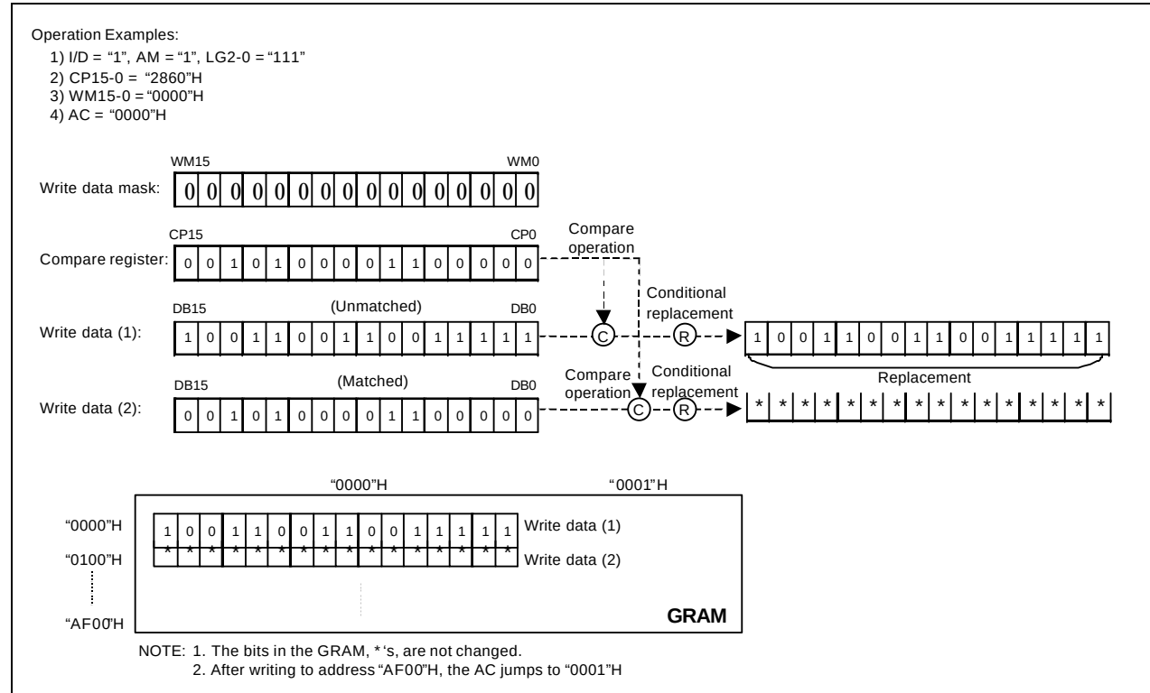
Figure 30. Writing operation of write mode 4
