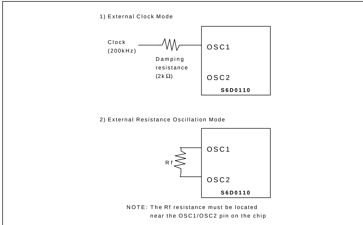
Figure 47. Oscillation Circuit
