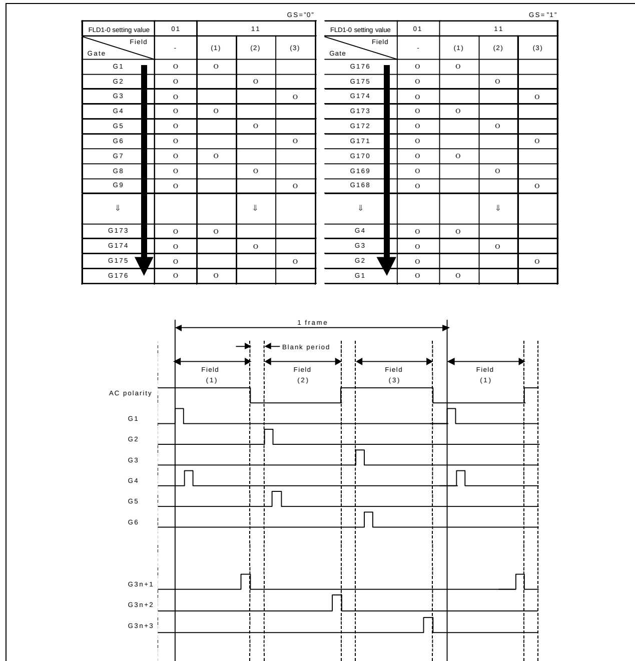
Figure 49. Interlace drive and output waveform
