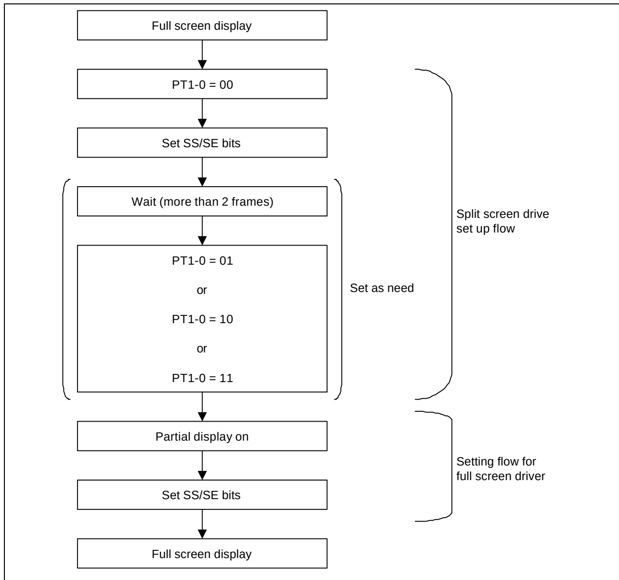
Figure 53. Partial display set up flow
