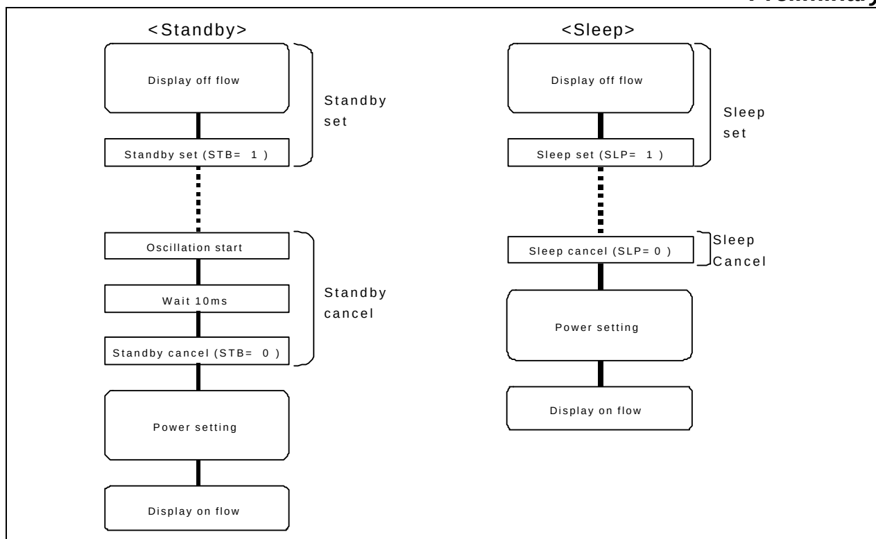
Figure 46. Instruction setup flow (continued)
