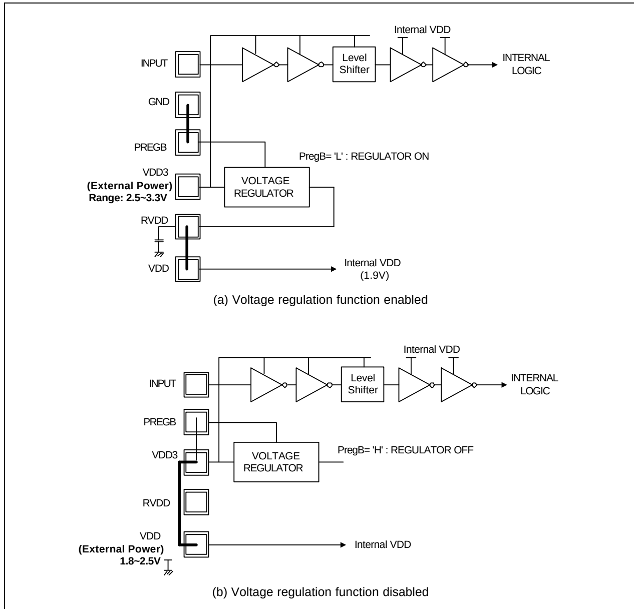
Figure 13. Voltage regulation function
