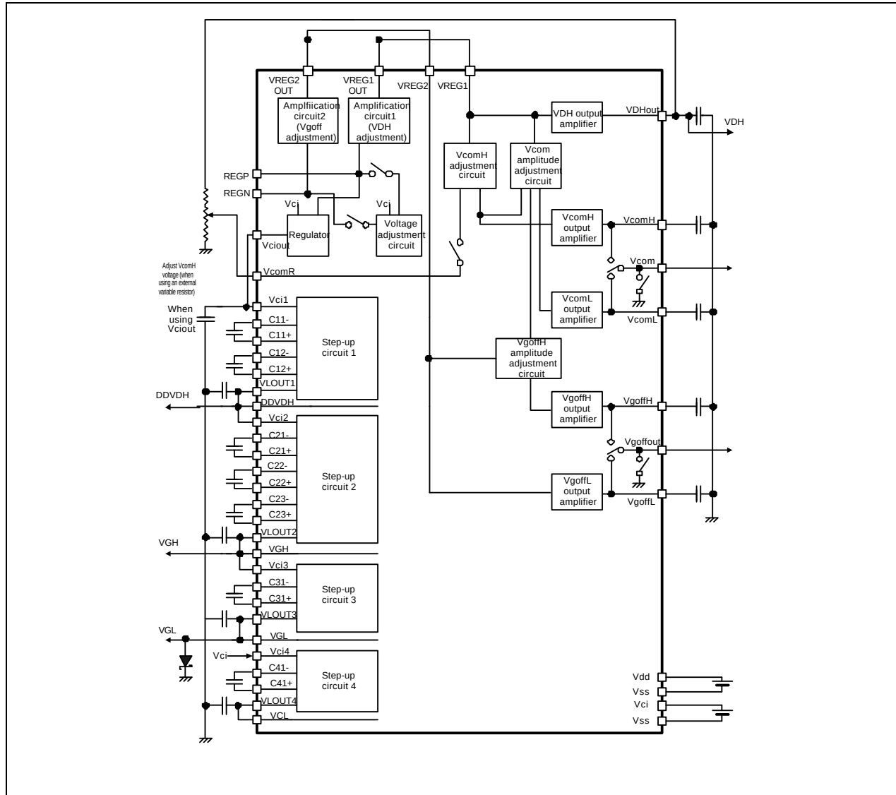
Figure 5. Configuration of the Internal Power-Supply Circuit
