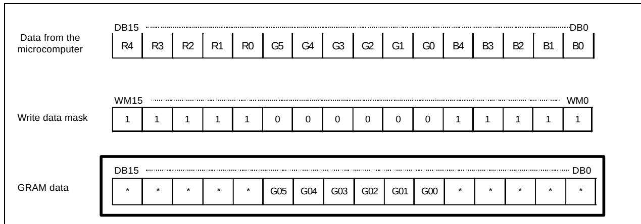
Figure 26. Example of write-data mask function operation
