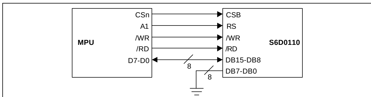
Figure 18. Interface to 8-bit microcomputer
