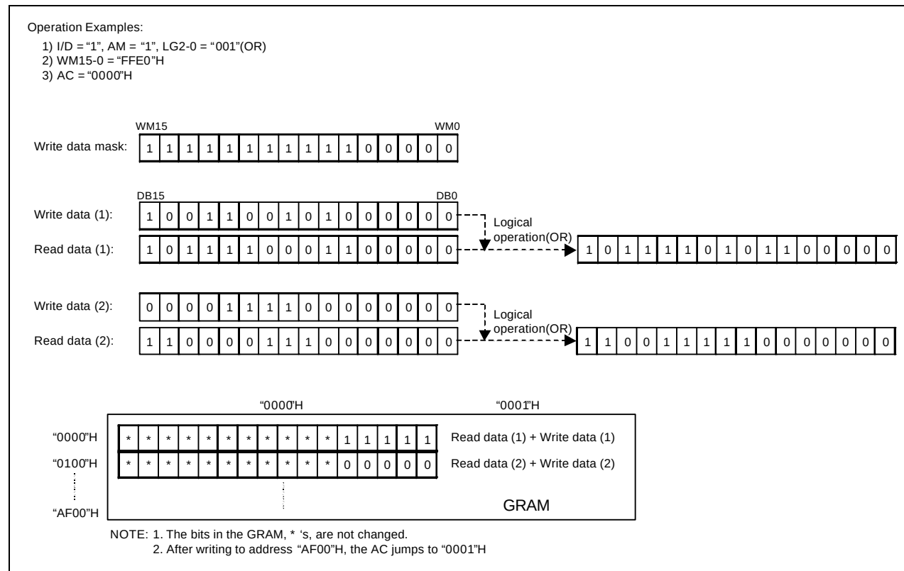
Figure 32. Writing operation of read/write mode 2
