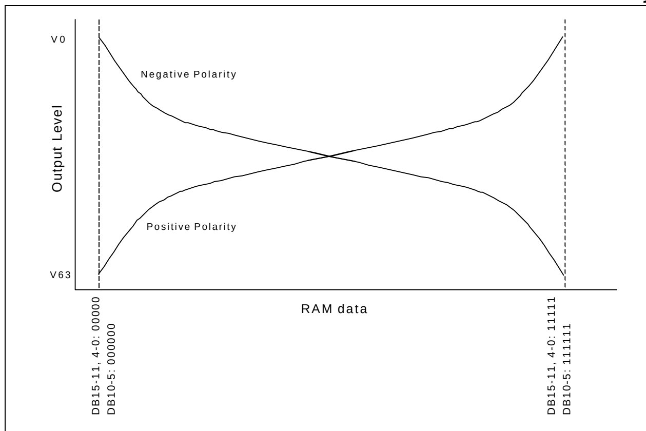
Figure 40. Relationship between RAM data and output voltage
