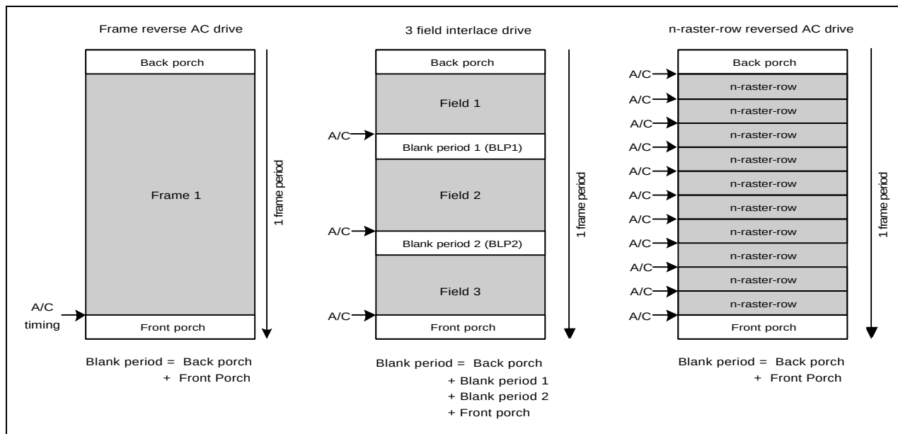
Figure 50. A/C timing
