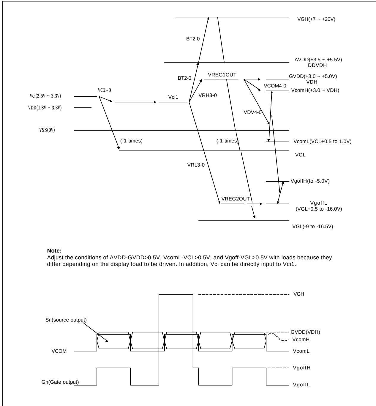
Figure 6. Pattern diagram and an example of waveforms
