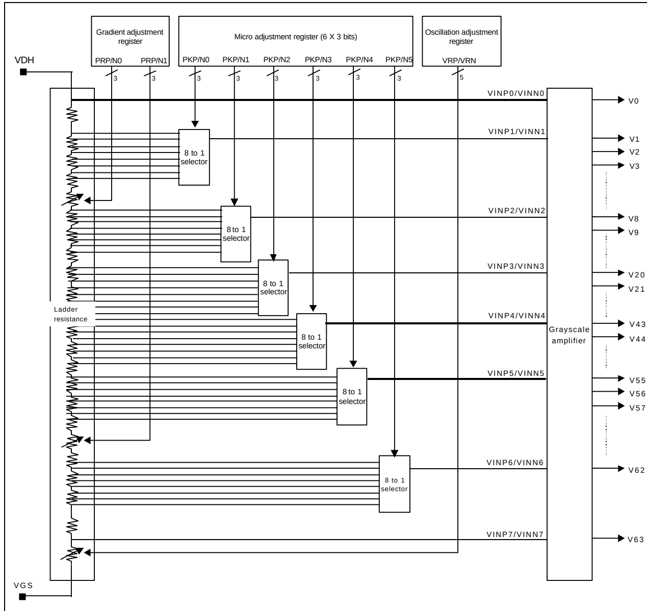
Figure 37. Structure of grayscale amplifier
