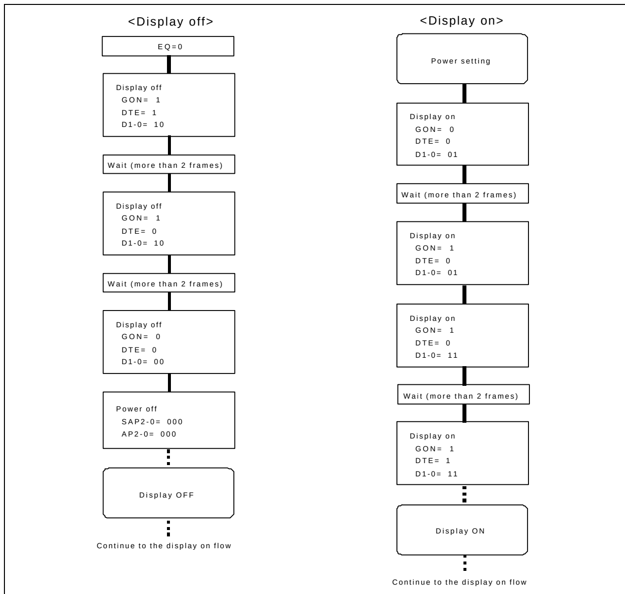
Figure 45. Instruction set up flow
