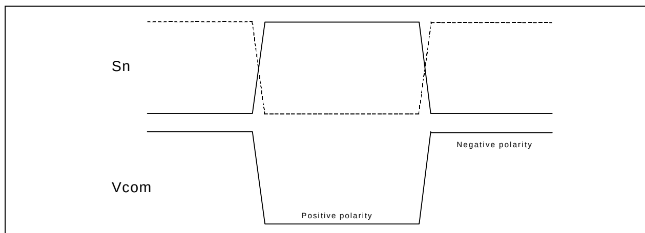
Figure 41. Relationship between source output and V_{com}
