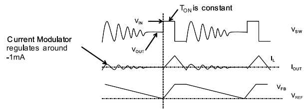
Figure 3: Light-Load Operation
