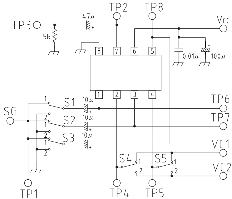
SOP-8C
