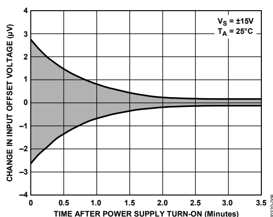
Figure 7. Warm-Up Drift
