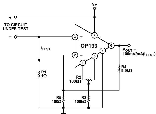
Figure 32. Single-Supply Current Monitor
