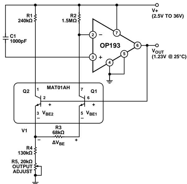
Figure 31. A Battery-Powered Voltage Reference
