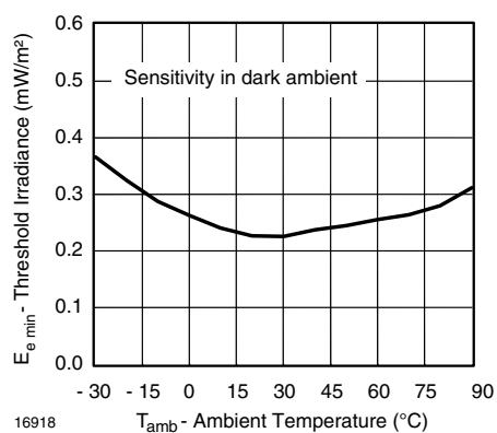
Figure 10. Sensitivity vs. Ambient Temperature
