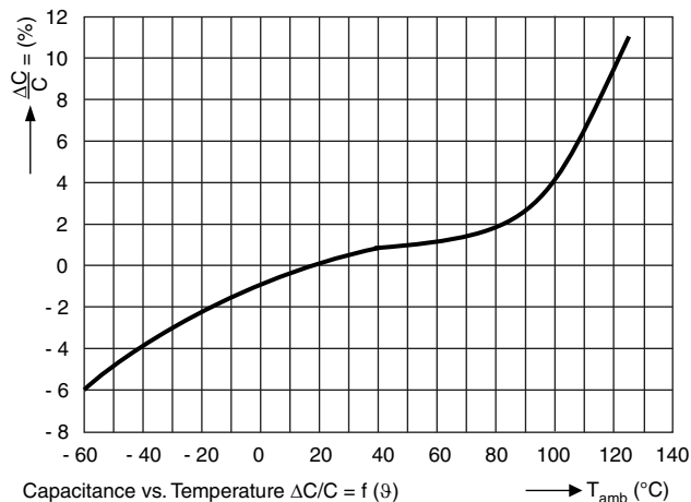
Capacitance vs. Temperature \Delta C/C = f(\vartheta) Capacitance as a function of temperature \Delta C/C = f(T_A), T_{LL} \leq T_A \leq T_{UL}
