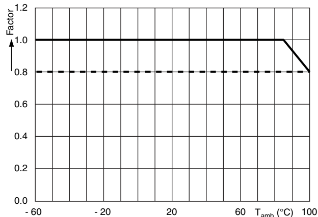
Nominal voltage (AC and DC) as a function of temperature U = f(T_A), T_{LL} \leq T_A \leq T_{UL}
