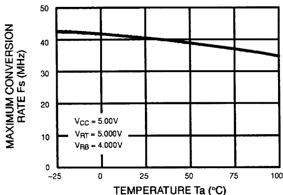
Fig. 16 – MAXIMUM CONVERSION RATE vs. TEMPERATURE
