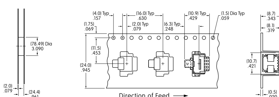
Tape Dimensions
