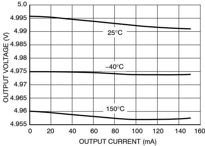
Figure 5. Output Voltage vs. Output Current (OUT = 5 V)
