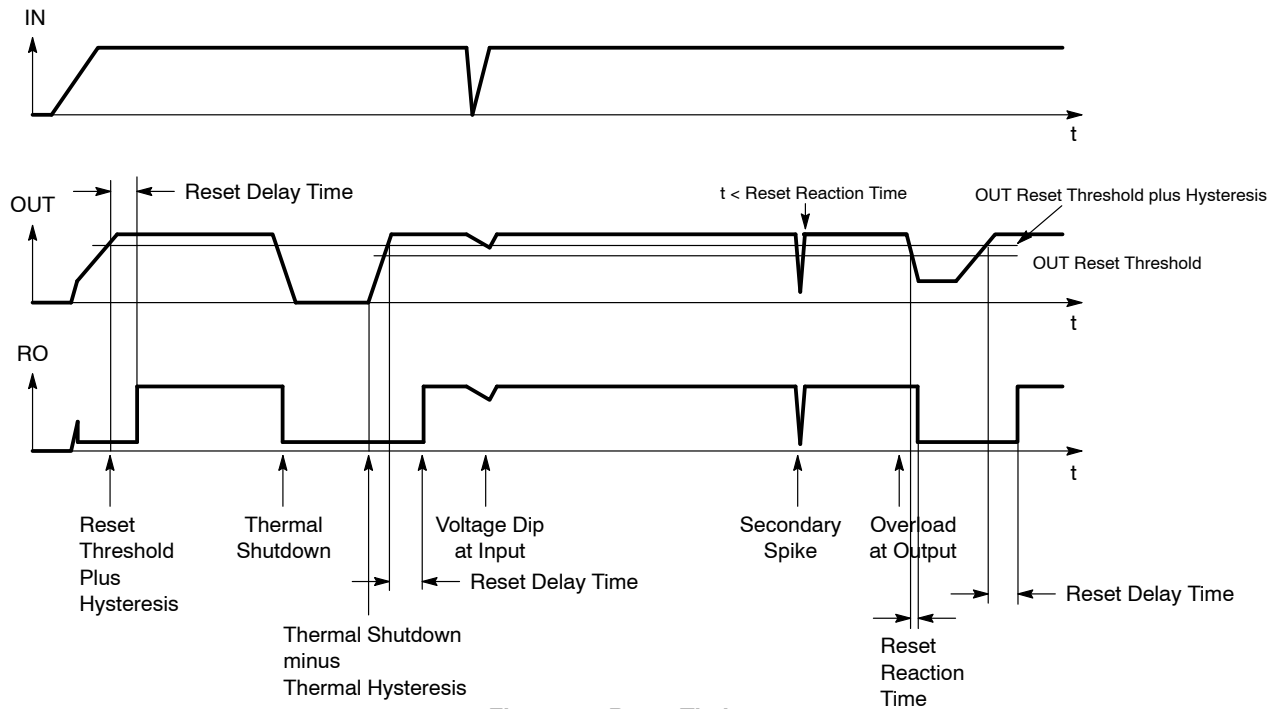
Figure 25. Reset Timing
