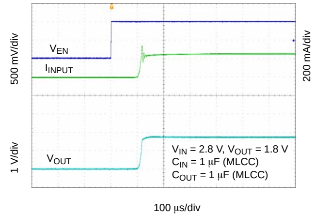
Figure 36. Enable Turn-on Response – C_{OUT} = 1\text{ μF} , I_{OUT} = 250\text{ mA}
