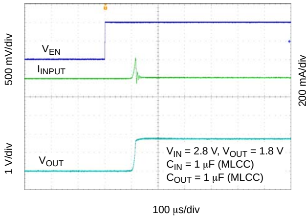
Figure 35. Enable Turn-on Response – C_{OUT} = 1\text{ μF} , I_{OUT} = 10\text{ mA}
