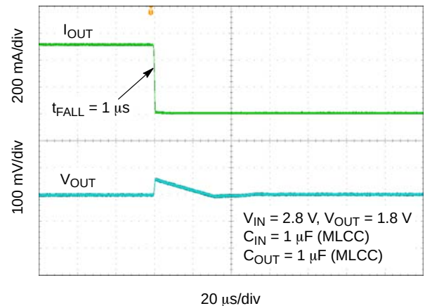
Figure 42. Load Transient Response – 450 mA to 1 mA – V_{OUT} = 1.8 \text{ V}
