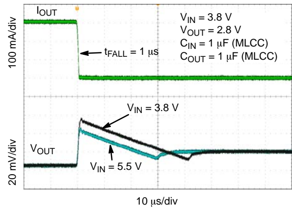
Figure 39. Load Transient Response – Falling Edge, V_{OUT} = 2.8 V , I_{OUT} = 1 mA to 300 mA, V_{IN} = 3.8 V , 5.5 V
