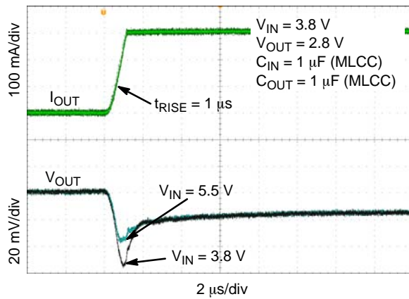
Figure 38. Load Transient Response – Rising Edge, V_{OUT} = 2.8 V , I_{OUT} = 1 mA to 300 mA, V_{IN} = 3.8 V , 5.5 V
