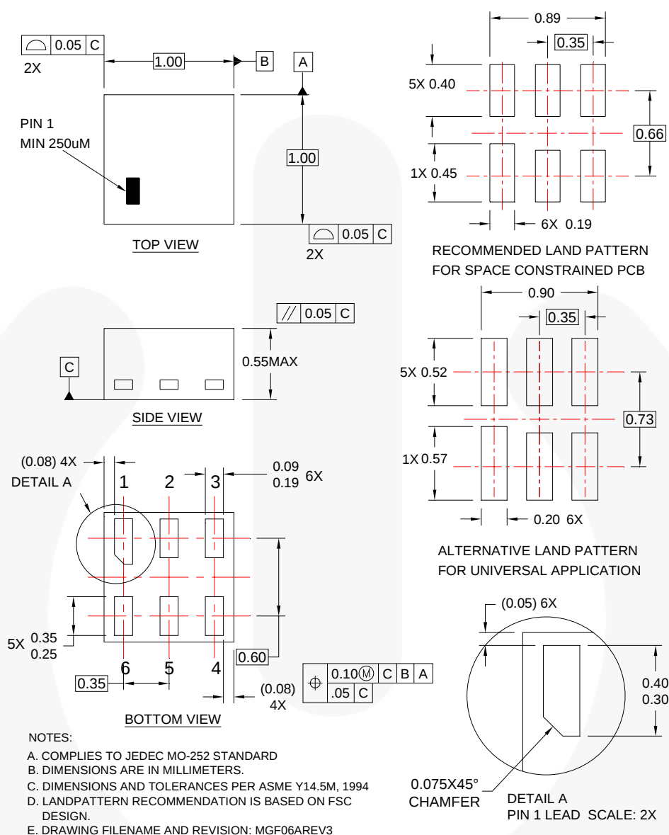
Figure 9. 6-Lead, MicroPak2, 1x1mm Body, .35mm Pitch
