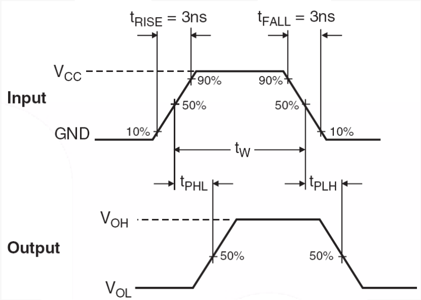
Figure 6. AC Waveforms
