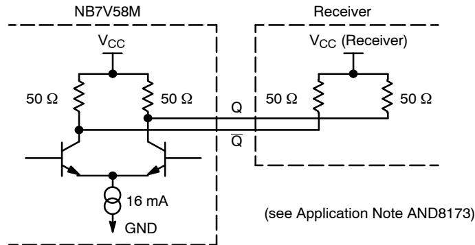
Figure 16. Typical CML Output Structure and Termination
