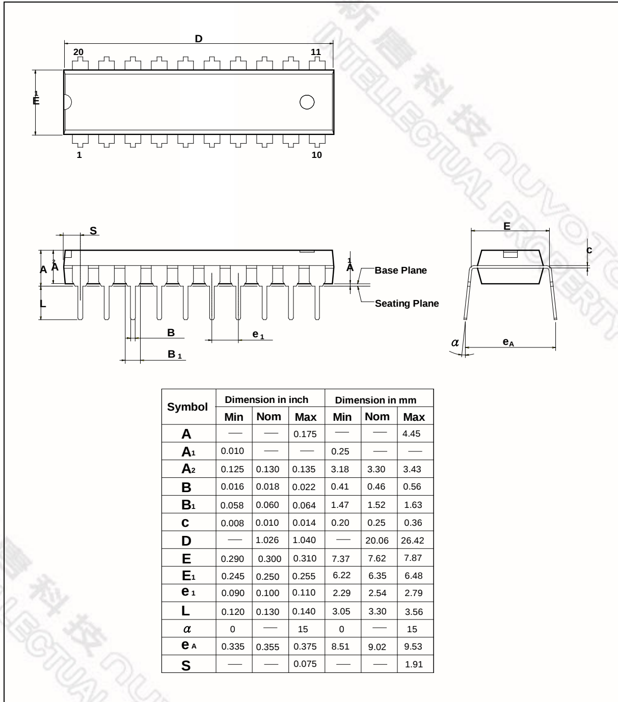
Figure 27-2: 20L DIP-300mil
