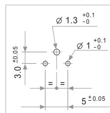
PCB Hole Layout
