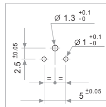
PCB Hole Layout
