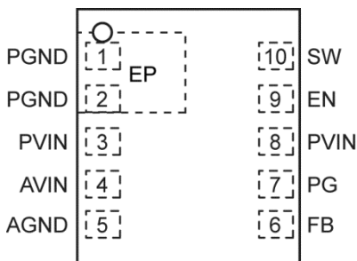
3mm × 4mm DFN (FL) (Top View)
