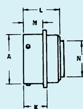
Crimp KPSE02/MS3122
