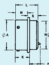
Solder KPT02/MS3112
