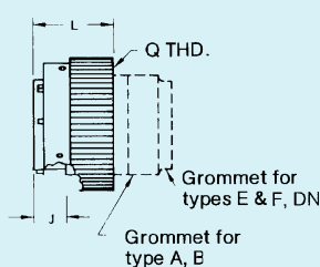
Crimp KPSE06/MS3126
