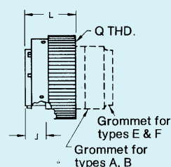
Crimp KPSE08
