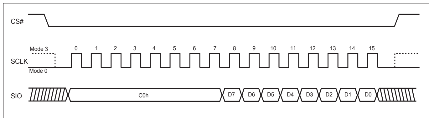
Figure 38. SPI Mode
