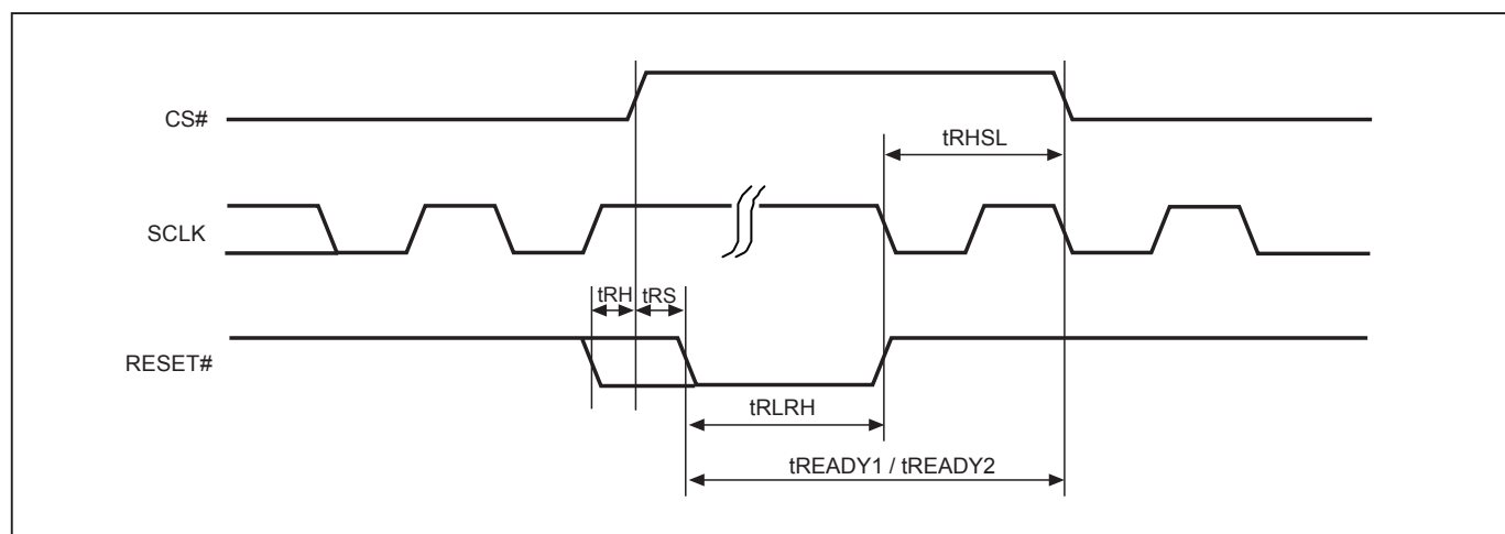
Figure 82. RESET Timing
