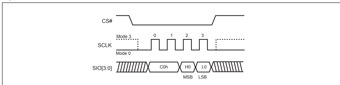
Figure 39. QPI Mode
