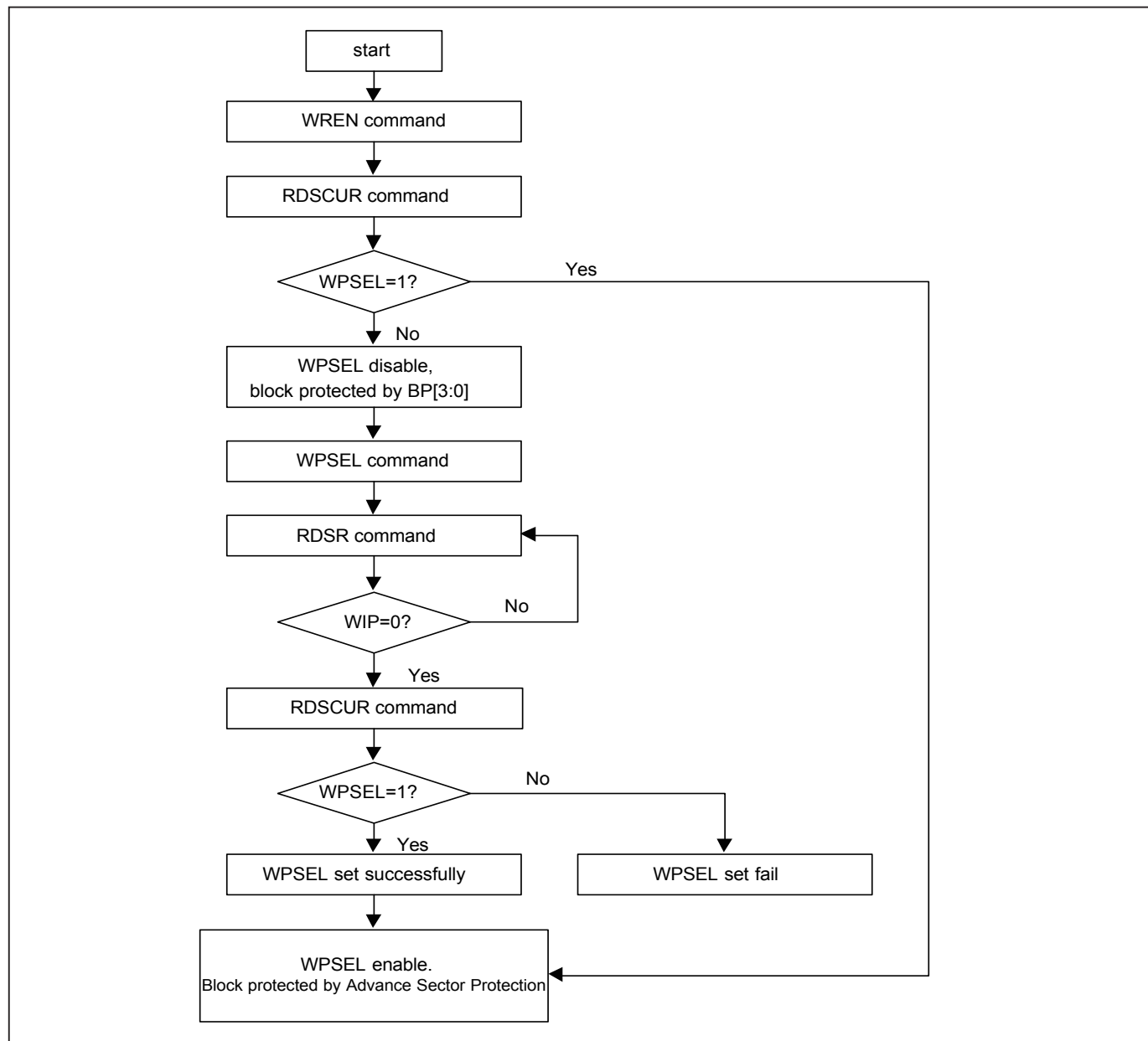
Figure 64. WPSEL Flow
