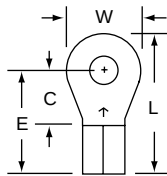
MU10-6R Stud Size 6 Wire Range 12-10
