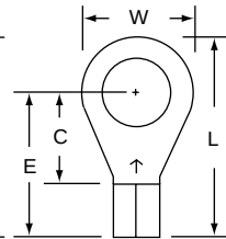
MU10-516R/S Stud Size 5/16 Wire Range 12-10
