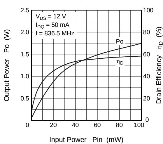
Output Power, Drain Efficiency vs. Input Power
