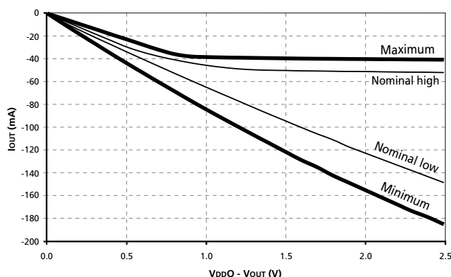
Figure 6: Pull-Up Characteristics
