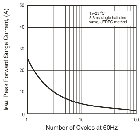
Fig.3- Typical Reverse Characteristics Forward Surge Current
