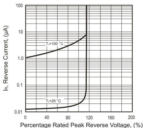
Fig.5- Maximum Non-repetitive
