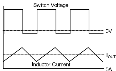
Figure 2. Continuous Operation
