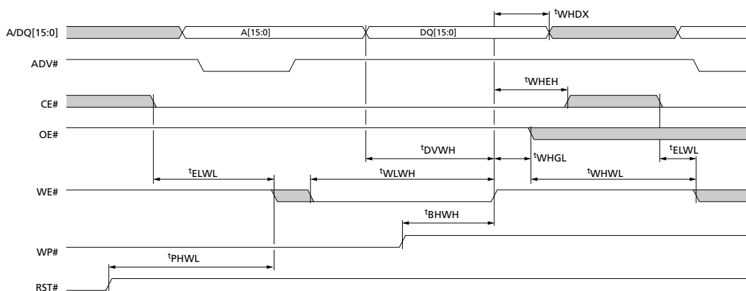
Figure 58: AADM Asynchronous WRITE Cycle (Latching A[15:0] only)
