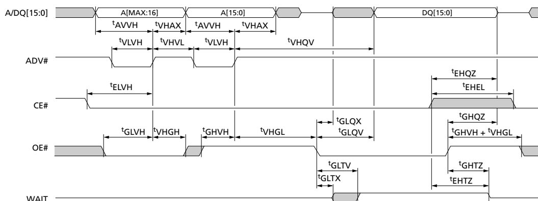
Figure 55: AADM Asynchronous READ Cycle (Latching A[15:0])
