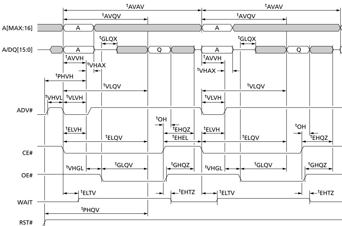
Figure 27: Asynchronous Single-Word Read
