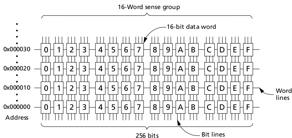
Figure 6: Wrap/No-Wrap Example
