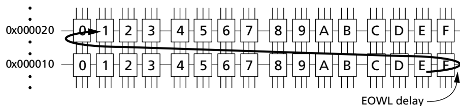
Figure 7: End-of-Wordline Delay
