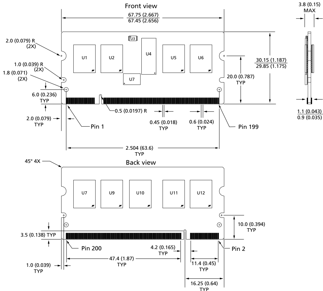
Figure 5: 200-Pin DDR2 SODIMM
