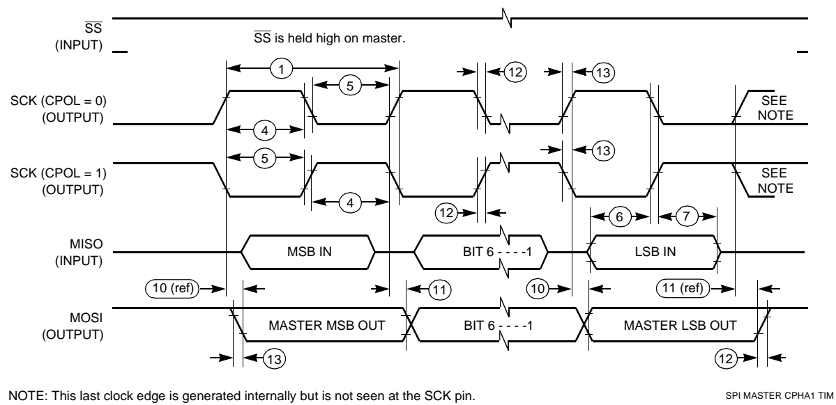
Figure A-10 SPI Master Timing (CPHA = 1)
