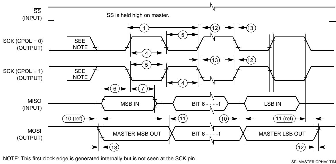
Figure A-9 SPI Master Timing (CPHA = 0)
