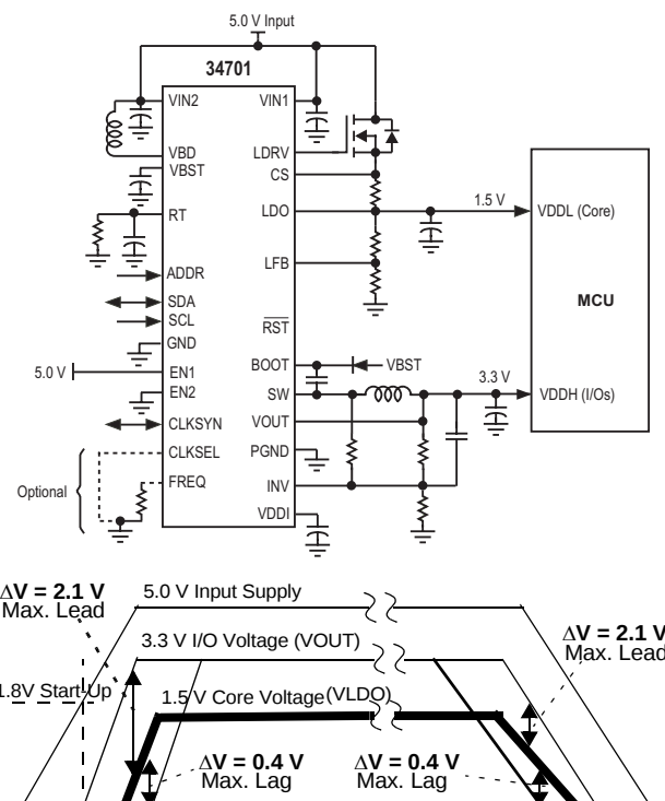
Figure 19. Inverted Power Up/Down Sequence in +5.0 V Supply System
