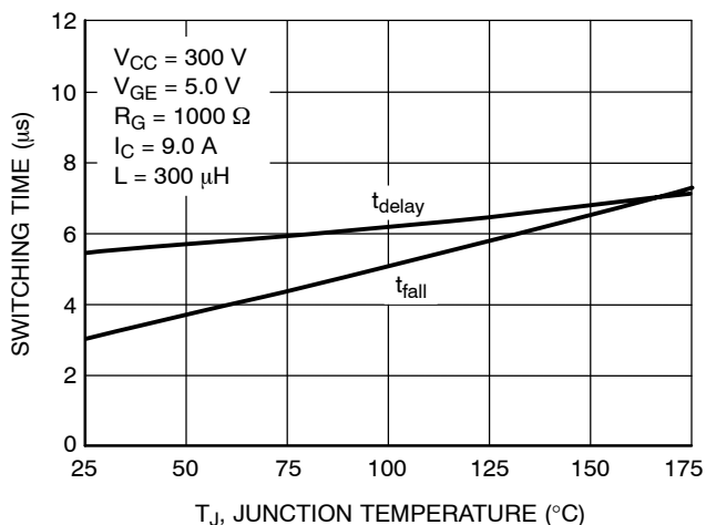
Figure 12. Inductive Switching Fall Time vs. Temperature
