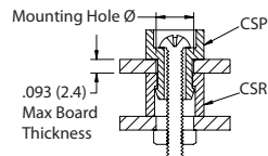
Typical Assembly
