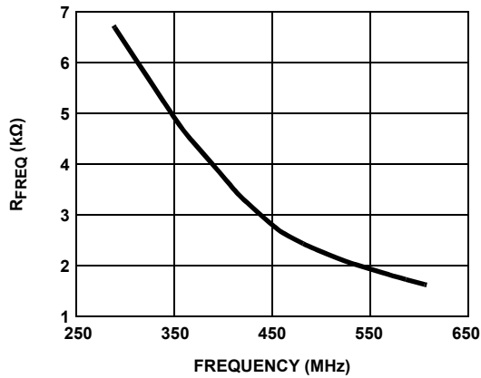
FIGURE 4. FREQUENCY CONTROL
