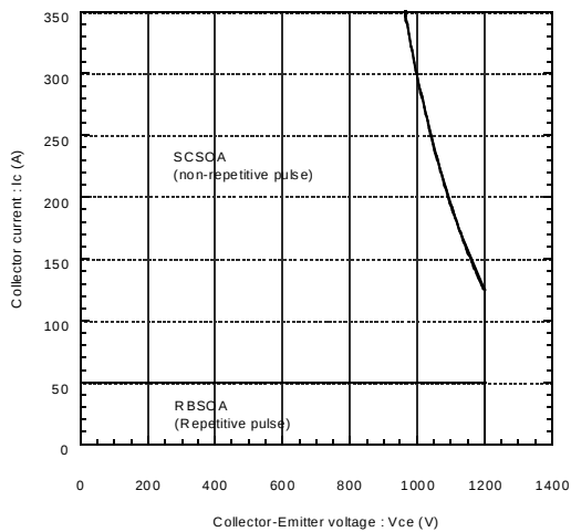
Reversed biased safe operating area V_{cc}=15V, T_j \leq 25^{\circ}C (min.)
