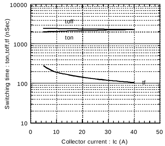
Switching time vs. Collector current (typ.) E_{dc}=600V, V_{cc}=15V, T_j=125^{\circ}C
