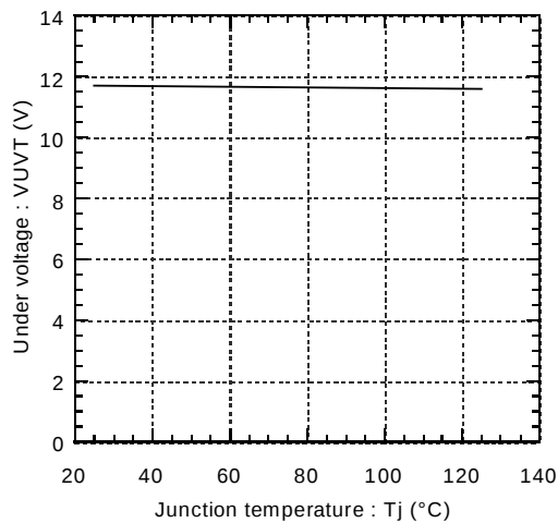
Under voltage vs. Junction temperature (typ.)
