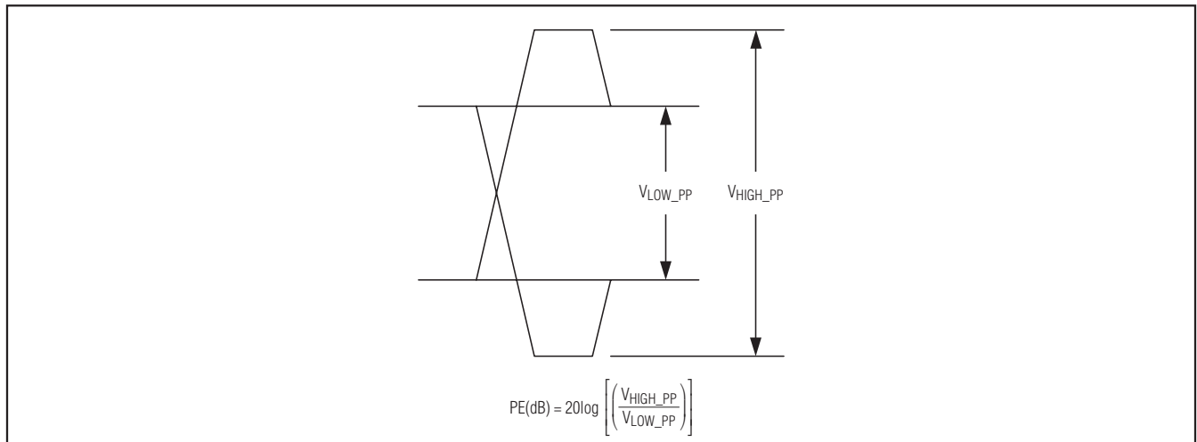
Figure 1. Output Preemphasis
