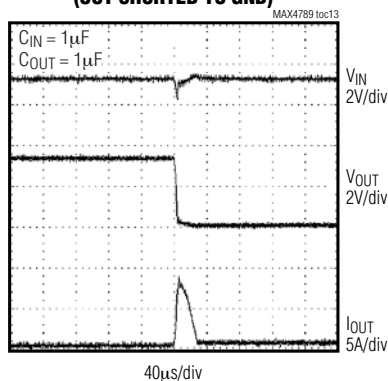
CURRENT-LIMIT RESPONSE (OUT SHORTED TO GND)
