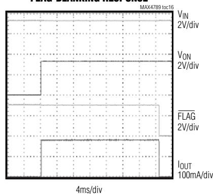
FLAG-BLANKING RESPONSE
