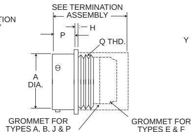
CRIMP KPSE01/MS3121
