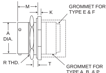
CRIMP KPSE07/MS3124
