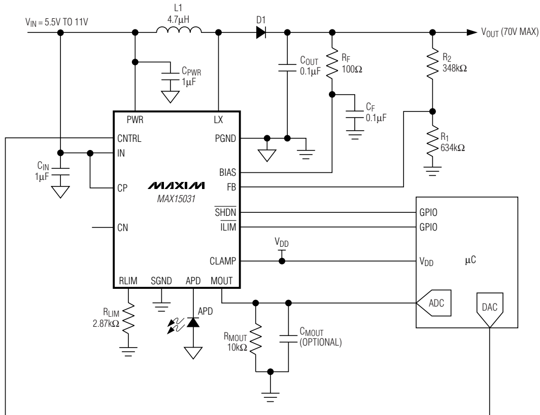
Figure 4. Typical Operating Circuit for V_{IN} = 5.5V to 11V
