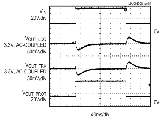
LINE-TRANSIENT RESPONSE
