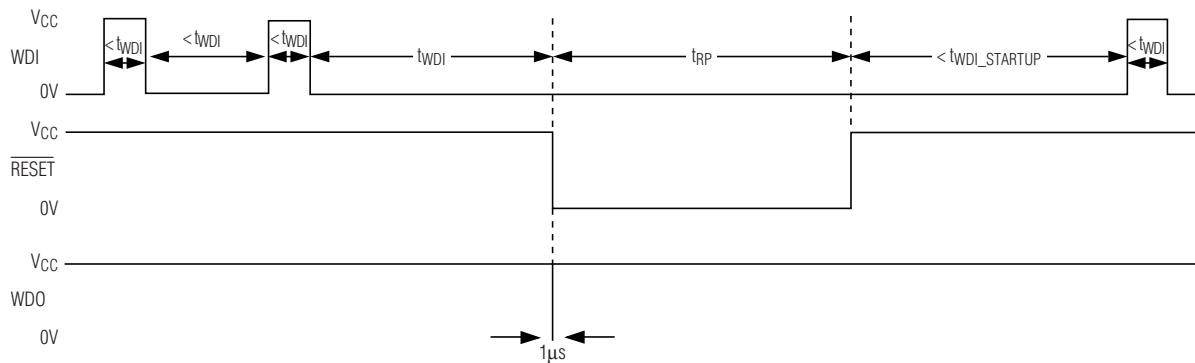
Figure 8. Watchdog Startup Sequence with Watchdog \overline{RESET} Enable Bit (r55h[7]) Set to '1'
