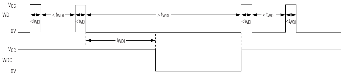
Figure 7. Watchdog Timer Operation
