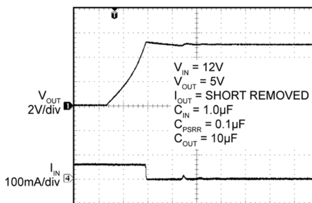
Short-Circuit Output Voltage Recovery
