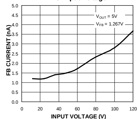
FB Current vs. Input Voltage
