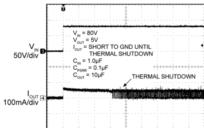
Thermal Shutdown, Short Circuit
