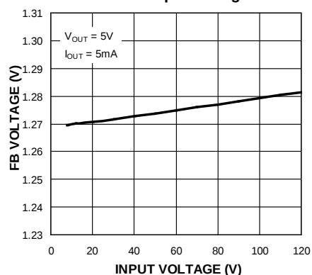
FB Voltage vs. Input Voltage
