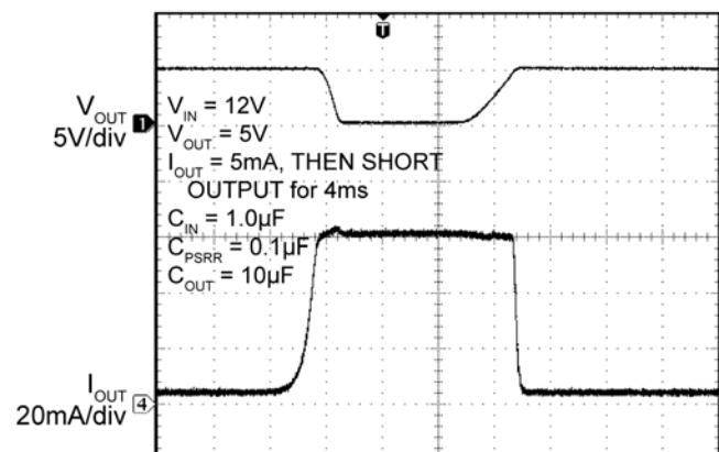
Current Limit
