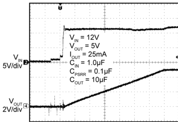
Hot Plug
