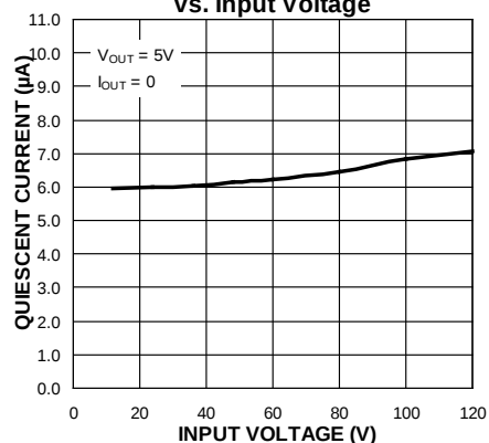
Quiescent Supply Current vs. Input Voltage
