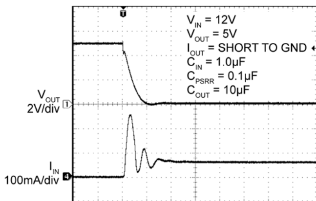
Short-Circuit Response
