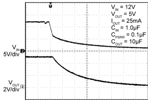
Hot Un-Plug
