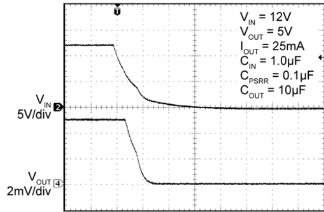
Soft Turn-Off
