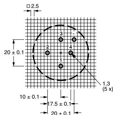
Case Ø D = 40 mm
