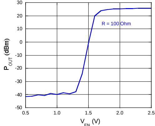
P_{OUT} vs. V_{EN} @ 2.4 V, 1900 MHz, P_{IN} = 0 dBm
