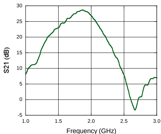
S21 vs. Frequency @ V_{CC} = 2.4 V, V_{EN} = 2.5 V
