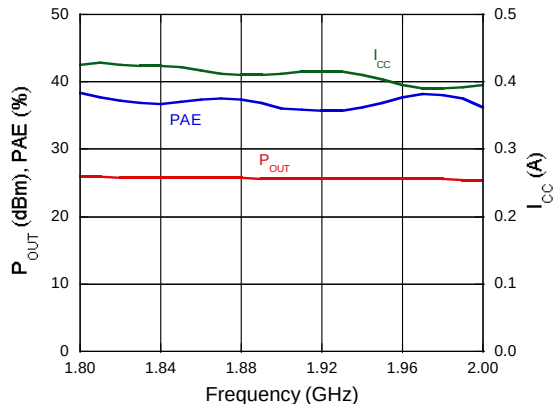
P_{OUT} , PAE, I_{CC} vs. Freq. @ 1900 MHz, P_{IN} = 0 dBm
