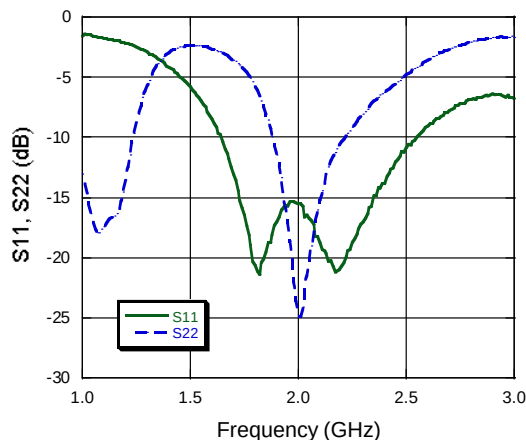
S22, S11 vs. Frequency @ V_{CC} = 2.4 V, V_{EN} = 2.5 V
