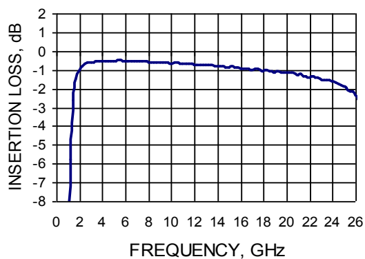
INSERTION LOSS vs FREQUENCY MA4SW310B-1
