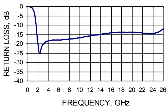
RETURN LOSS vs FREQUENCY MA4SW310B-1
